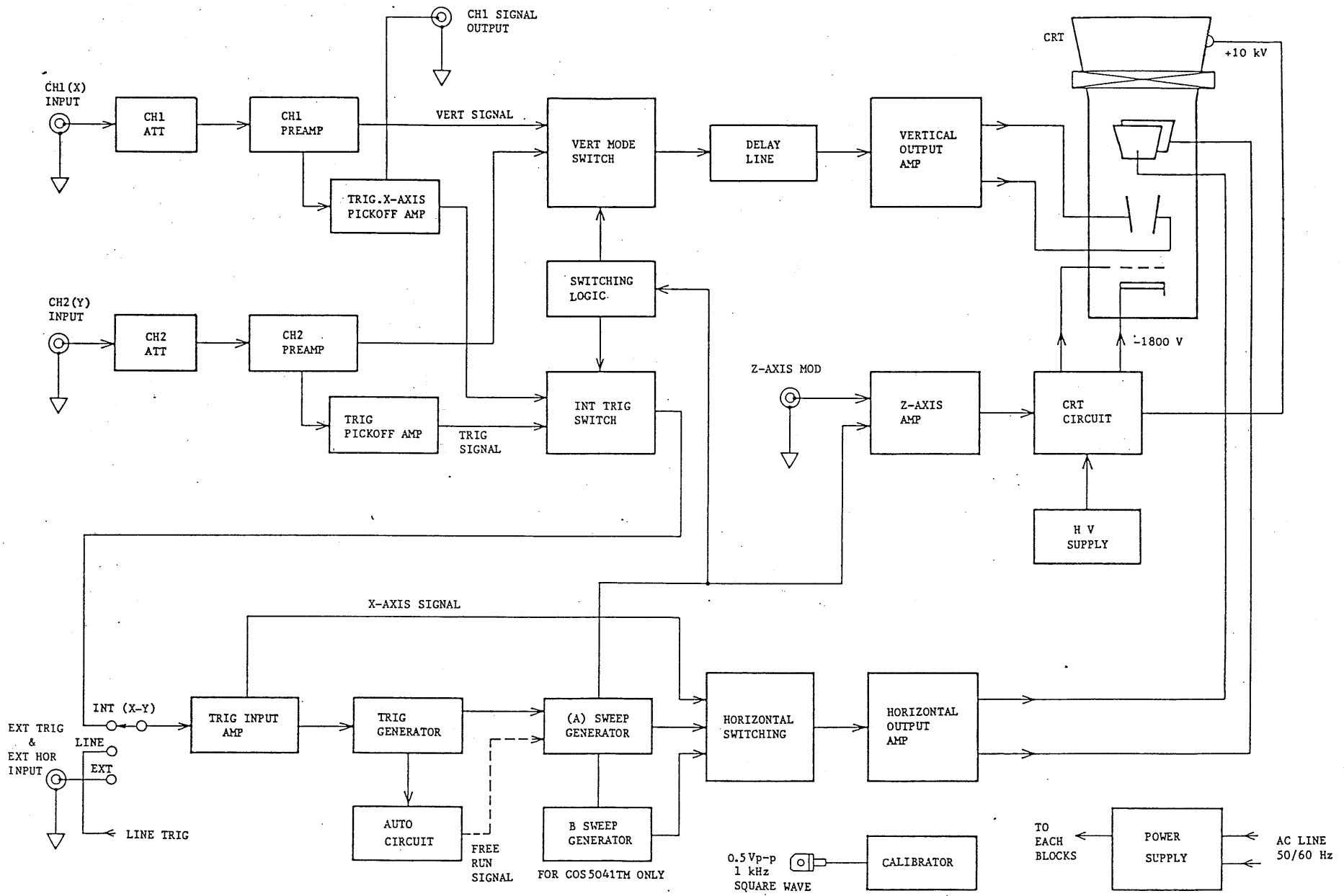
BLOCK DIAGRAM
